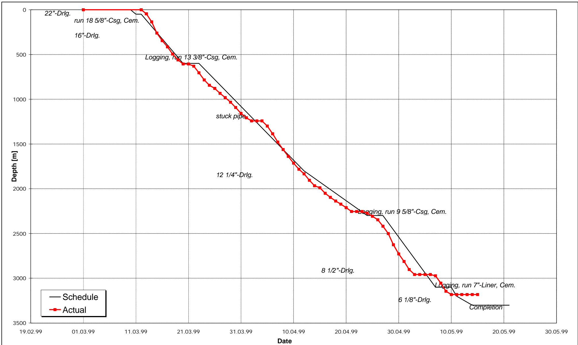
Example Well Time- vs. Depth-Curve Comparison Scheduled - Actual
