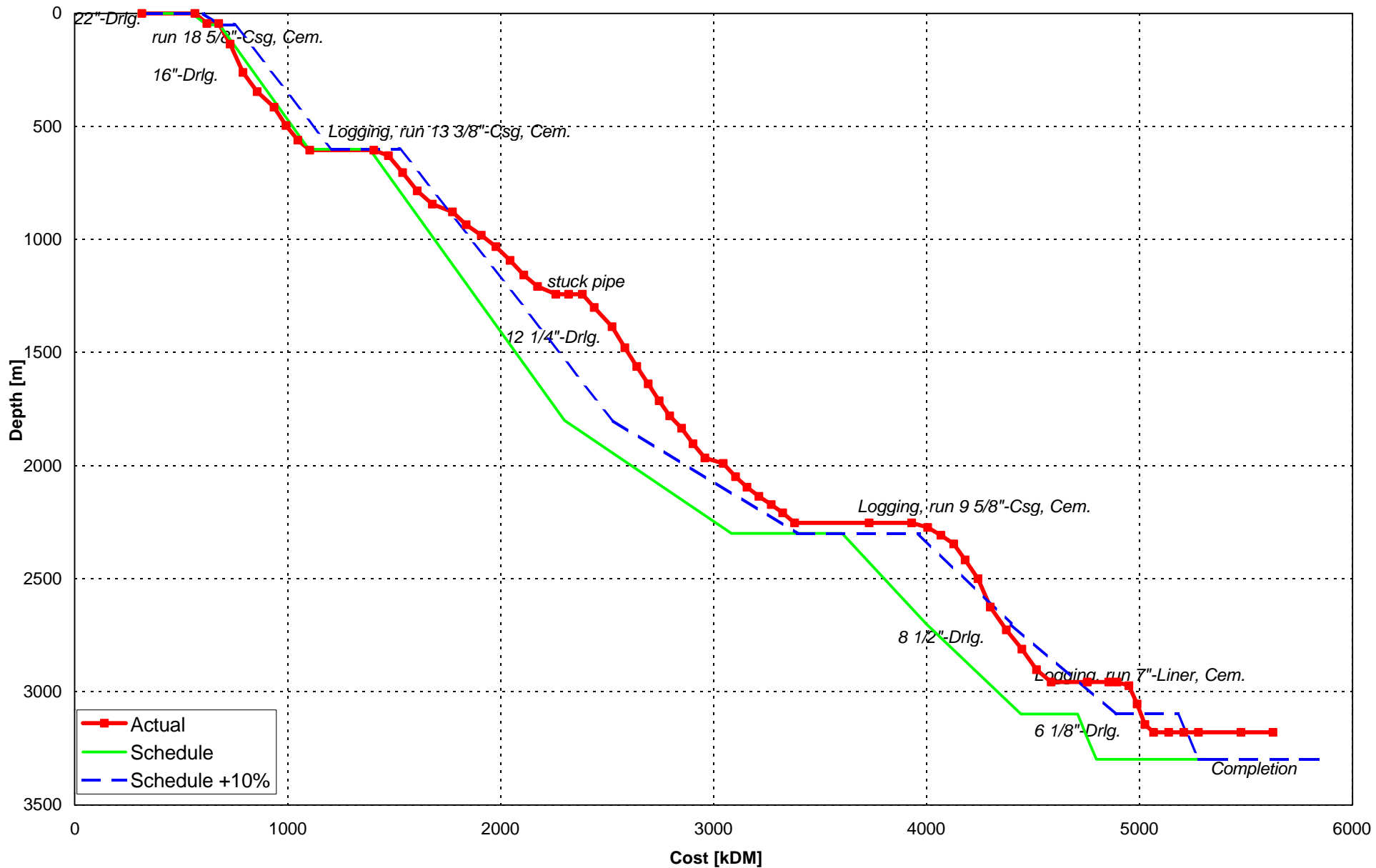
Example Well Cost- vs. Depth-Curve Comparison Scheduled - Actual
